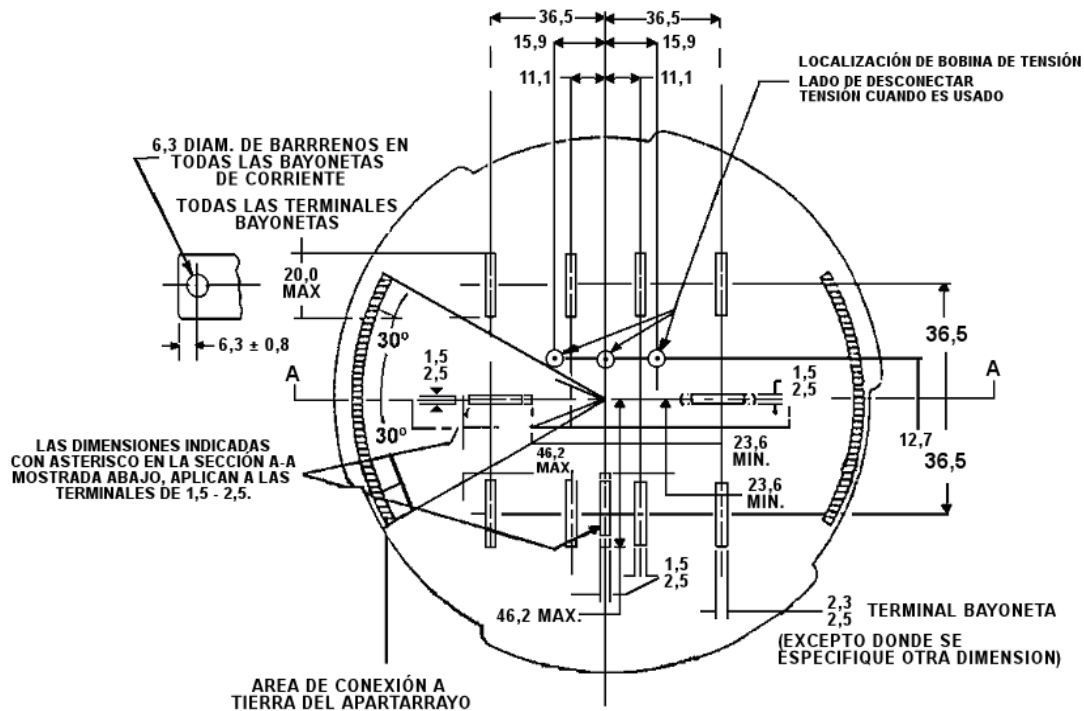
VISTA FRONTAL
